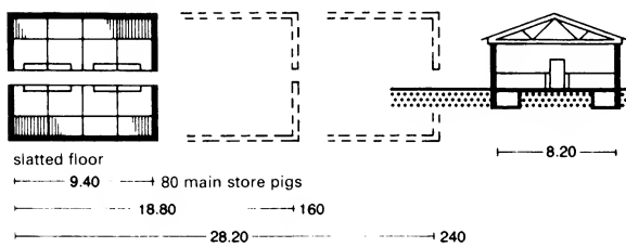
③ Store pig shed: two rows, long stalls, automatic feeding
